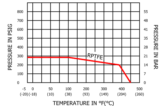
Pressure VS. Temperature Chart
